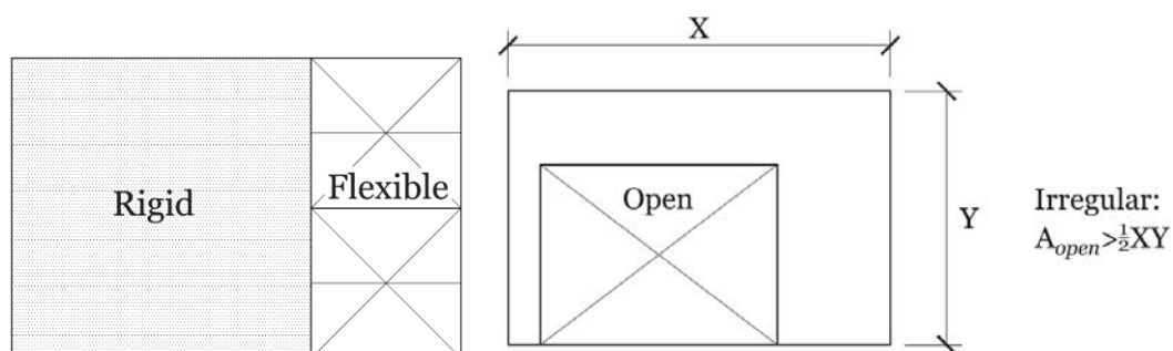
Figure 5-5: Diaphragm Discontinuity
