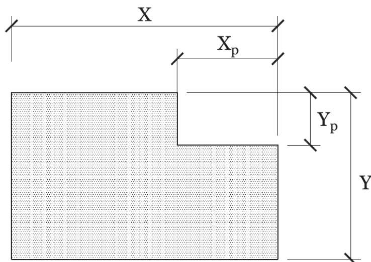
Figure 5-4: Re-entrant Corners
