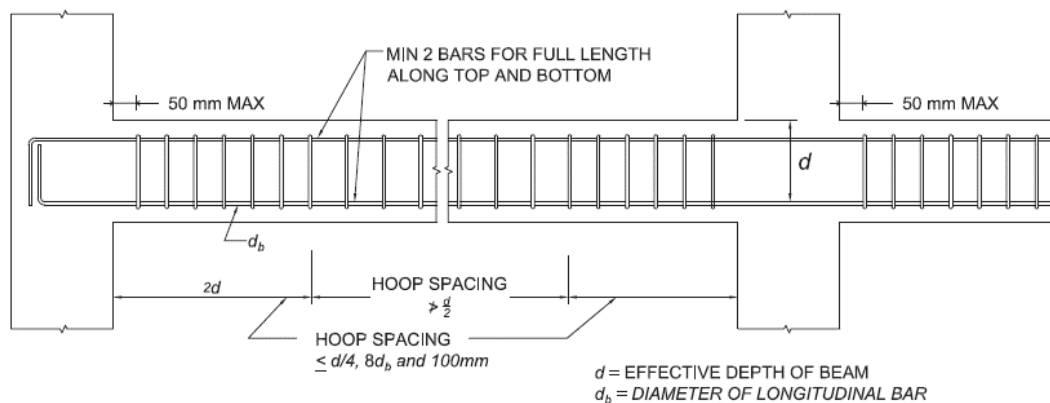
Figure 4-4 Details of transverse reinforcement in beams
