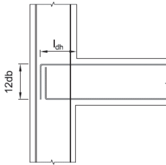
Figure 4-11 Anchorage of beam longitudinal bars in column
