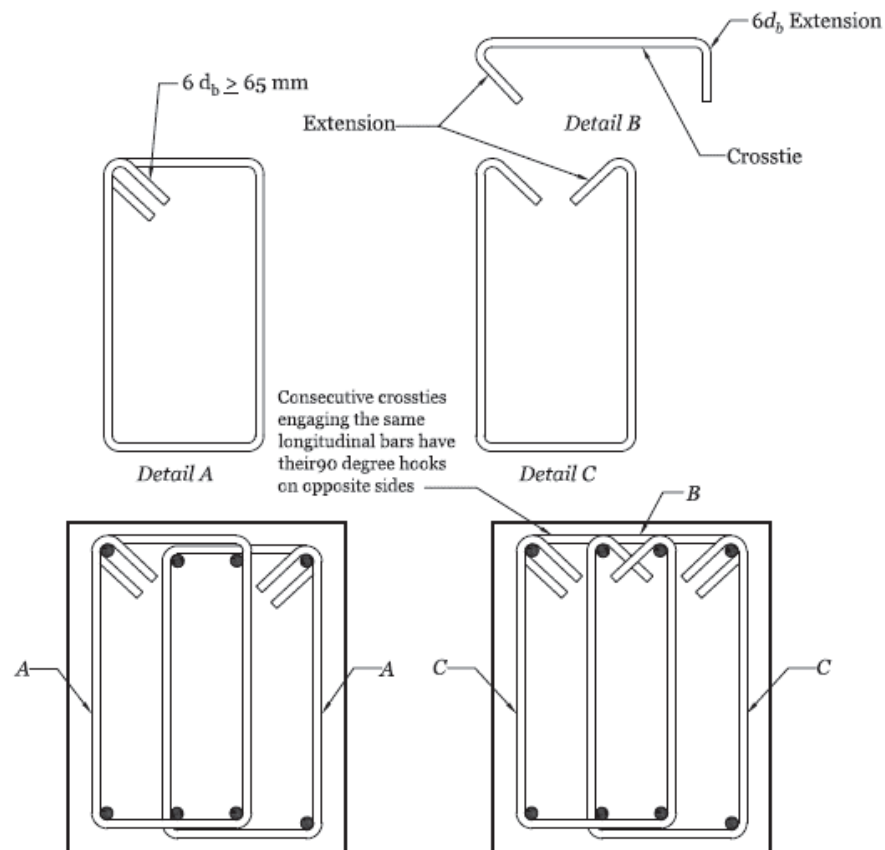
Figure 4-2 Details of Transverse reinforcement in beams
