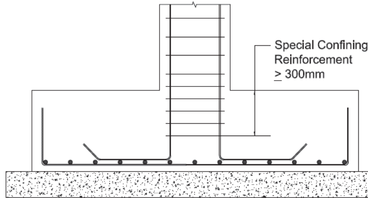
Figure 4-9 Confining reinforcement requirement in foundation
