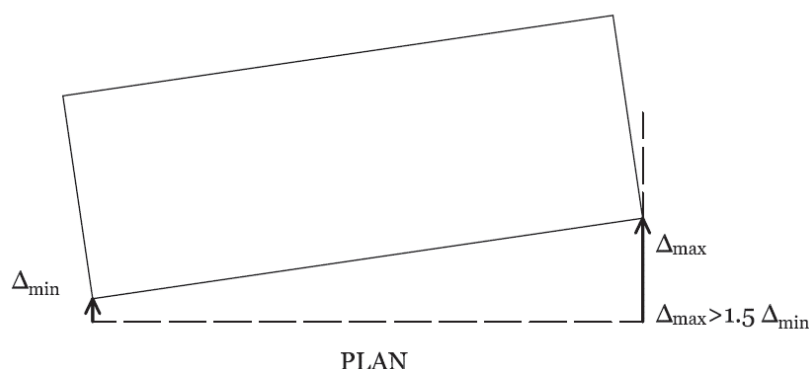
Figure 5-3: Torsion Irregularity
