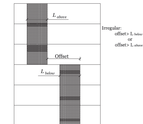
Figure 5-2: In-Plane Discontinuity
