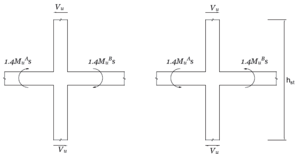
Figure 4-7 Calculation of Shear force demand in columns
