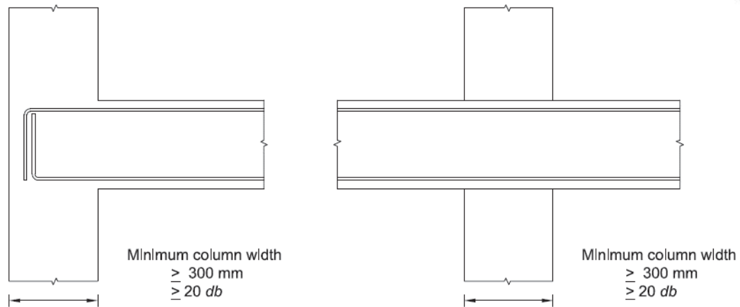
Figure 4-5 Requirement for minimum size of column member
