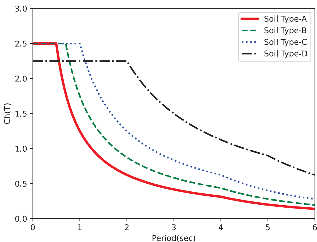
Figure 4-1 Spectral Shape Factor, C_h(T) for Equivalent Static Method
