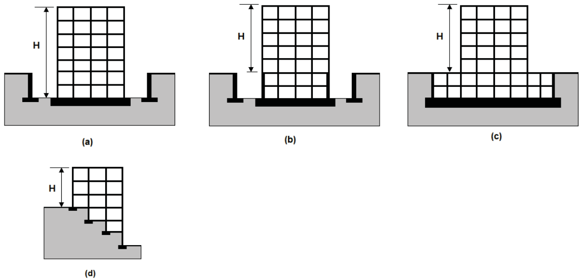
Figure 5-1: Height of Building
