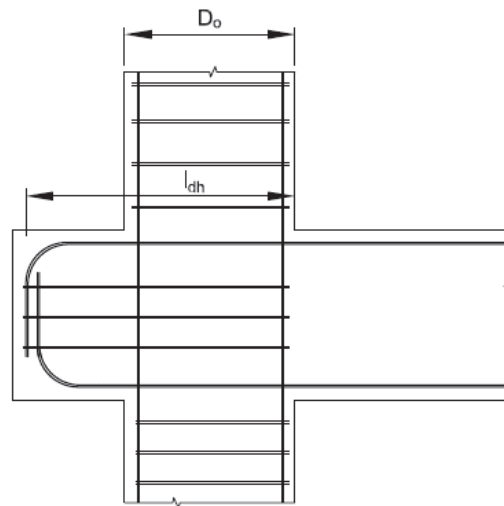
Figure 4-12 Provision of Beam stub
